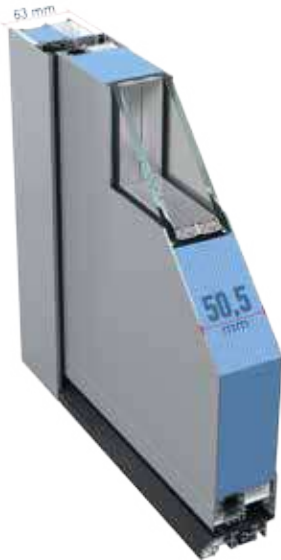
TLS50 FLATframe
